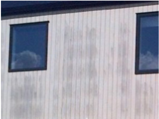
8.5 A New Zealand housing project with a very distinct batten (sub-frame) silhouette showing in the siding surface
